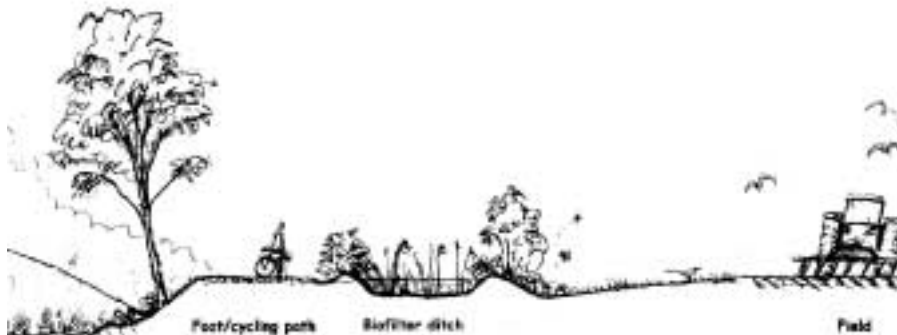
Principal section of the Vagnhärad pond system
