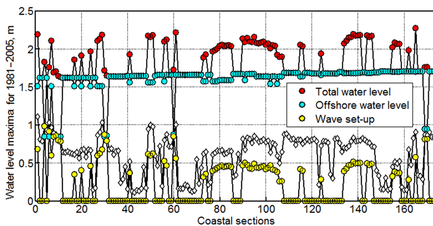
Fig. 4. The contribution of the hindcast instantaneous offshore water level and wave set-up into the all-time highest water level at the shoreline. The modelled all-time offshore water level maximum (not shown) varies insignificantly (from 1.6 m to 1.7 m) along the shore. White diamonds indicate the all-time highest wave set-up values. See Fig. 2 for the numbering of coastal sections.
