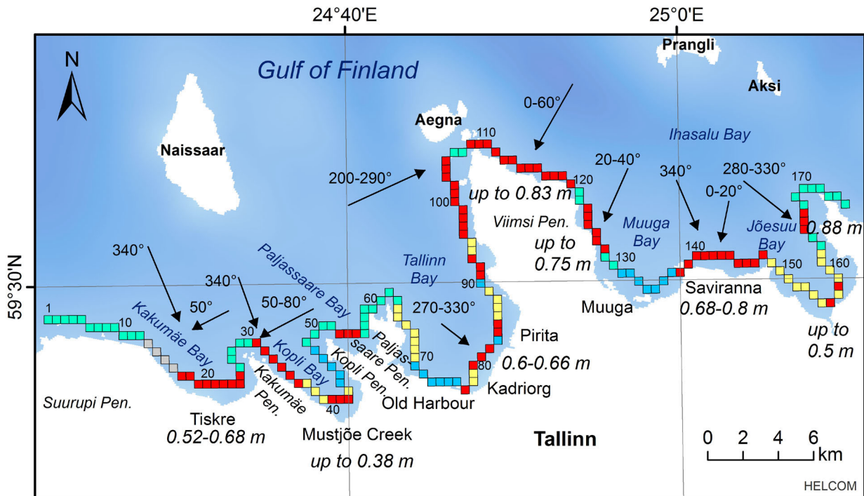
Fig. 2. Coastal sections potentially affected by high wave set-up (red squares) in the urban area of the City of Tallinn. The arrows indicate the associated directions of wave propagation. Yellow squares indicate coastal stretches where the maximum wave set-up is <20 cm, green squares are areas where high wave set-up is evidently not possible because of the convex shape of the shoreline, and blue squares refer to areas containing various engineering structures. Extended from [28] to cover areas to the east of the Viimsi Peninsula.
