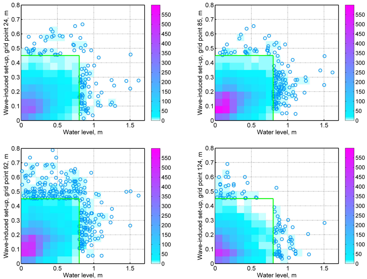
Fig. 3. Scatter diagrams of the occurrence of different offshore water levels and various wave set-up values at four representative sections of the study area: section 24 (Tiskre, a bayhead open to the north-west and partially to the west), section 85 (Pirita Beach, open only to the north-west), section 92 (western coast of the Viimsi Peninsula, open to the west), and section 124 (eastern coast of the Viimsi Peninsula, open to the north-east). The colour code corresponds to \geq 2 occasions (otherwise the area is left white) with a particular wave set-up (with a step of 0.05 m) and water level (with a step of 0.1 m). Single cases of wave set-up > 0.45 m and water levels > 0.8 m (outside of the rectangle bordered by green lines) are represented as separate circles. The situations with zero wave set-up (waves propagating offshore) and cases with offshore water levels below the long-term average are not shown.
