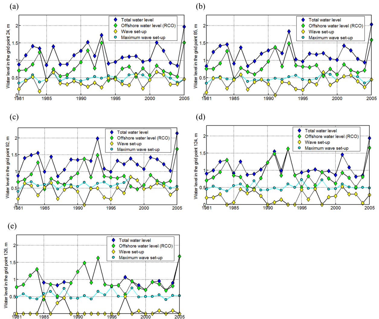
Fig. 5. The proportion of the wave set-up and offshore water level in the formation of annual maxima of the total water level at the shoreline at four representative sections of the study area: (a) Tiskre (section 24), (b) Pirita (85), (c) Viimsi (92), (d) Muuga (124), (e) a location close to Muuga Harbour (126) where wave set-up almost does not contribute. See Fig. 2 for the numbering of coastal sections.
