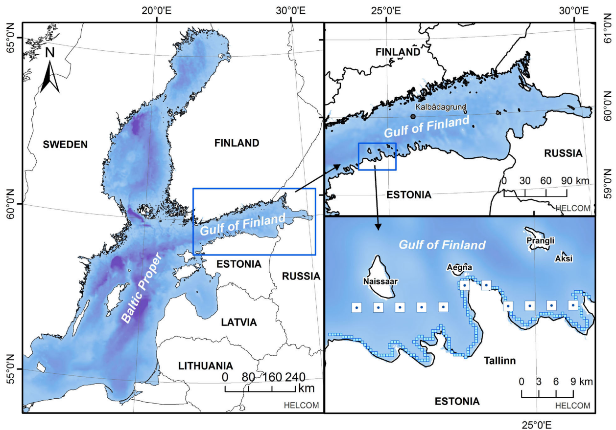
Fig. 1. Computational areas of the triple-nested wave model applied to the Tallinn Bay area. The small squares along the coast in the lower right panel indicate grid points of the wave model used in the analysis. The cells are numbered sequentially starting from the westernmost point (Fig. 2). The offshore water level is represented by 11 grid cells (white squares) of the RCO circulation model.
