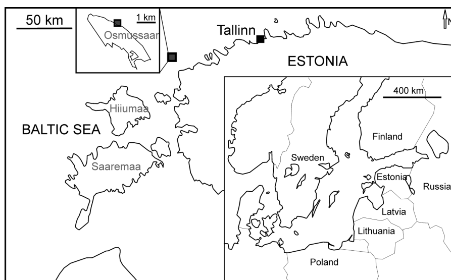
Fig. 1. Location of Osmussaar Island and locality of Oikobesalon traces.
