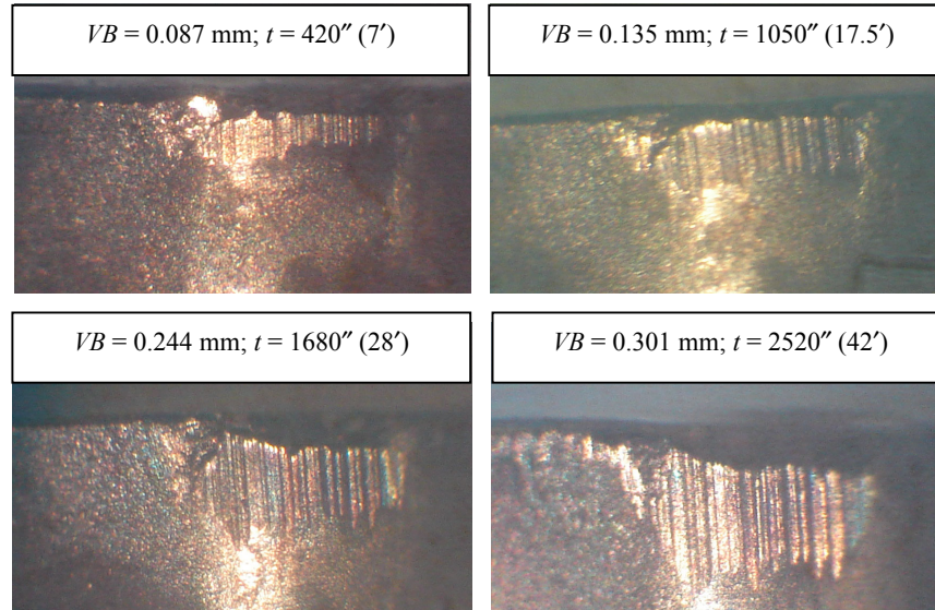
Fig. 5. Micrographs for VB of CC650 at a_p = 0.15 \text{ mm}; f = 0.16 \text{ mm/rev} and V_c = 120 \text{ m/min} .
